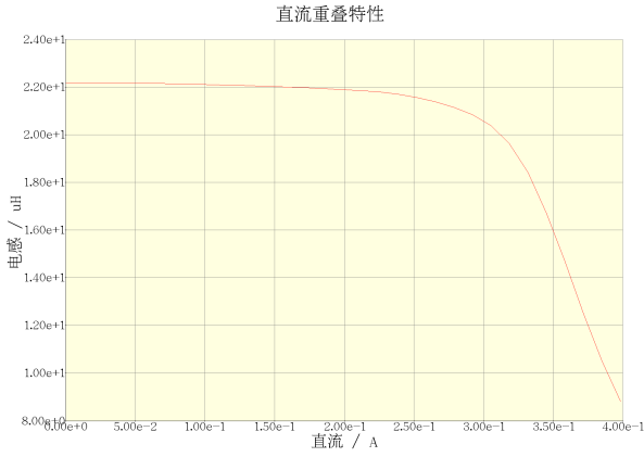
NLCV32T-220K-PF(Amb. Temp. = 20degc)
