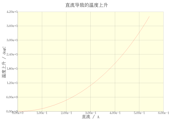
NLCV32T-220K-PF(Amb. Temp. = 20degc)
